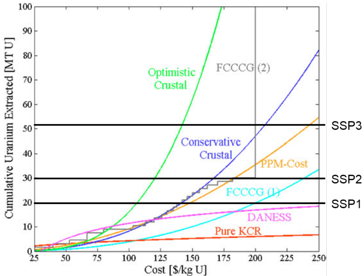
Fig. 3.2: Global uranium resources in the MESSAGE interpretation of the SSPs compared to seven supply curves from a literature review (Schneider and Sailor, 2008 [[100]]). Conservative Crustal and Optimistic Crustal refer to simple crustal models of uranium distribution in the crust and the of extraction costs on the concentration. Pure-KCR refers to a fit of a simple crustal model to known conventional resources (KCR) as estimated by the Red Book 2003 (OECD/NEA, 2004 [[116]]). PPM-Cost over the simple crustal models include a relationship between uranium grade and extraction costs. FCCCG(1) and (2) as well as DANESS refer to estimats from more complicated models of the dependency of extraction costs on uranium concentration (and therefore resource grade).
