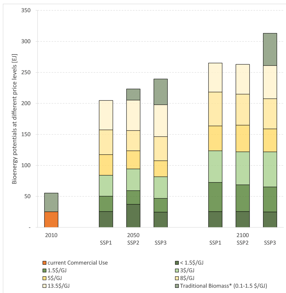
Fig. 3.3: Global bioenergy potential. Availability of bioenergy at different price levels in the MESSAGE-GLOBIOM model for the three SSPs (Fricko et al., 2017 [[17]]). Typically non-commercial biomass is not traded or sold, however in some cases there is a market – prices range from 0.1-1.5$/GJ (Pachauri et al., 2013 [[69]]) ($ equals 2005 USD).
