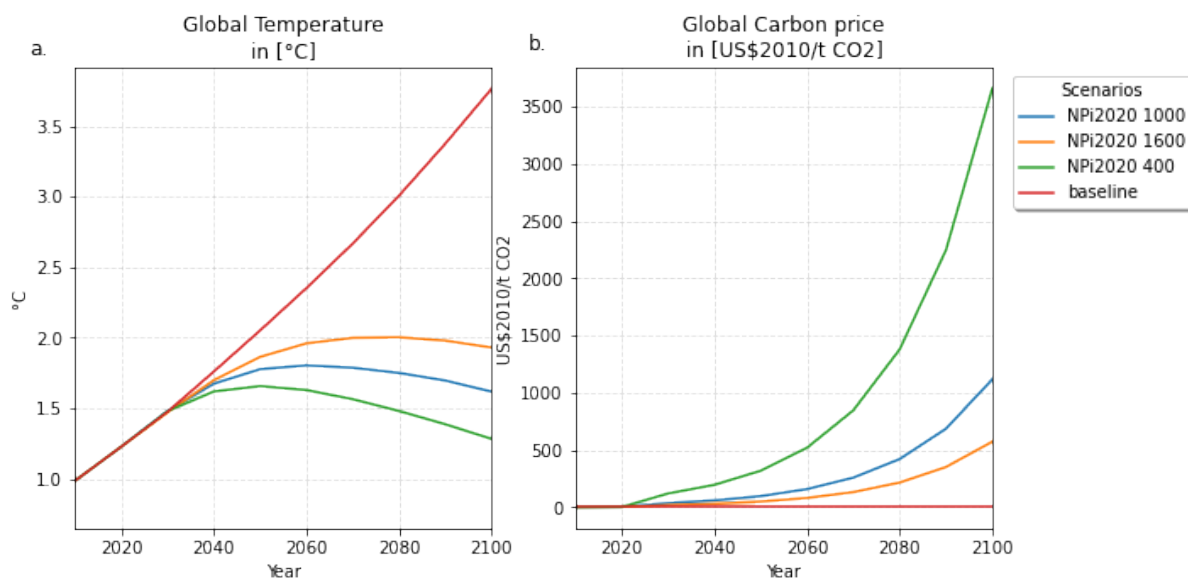
Fig. 5.8: Temperature and carbon-price development across CD-Links scenario set.
