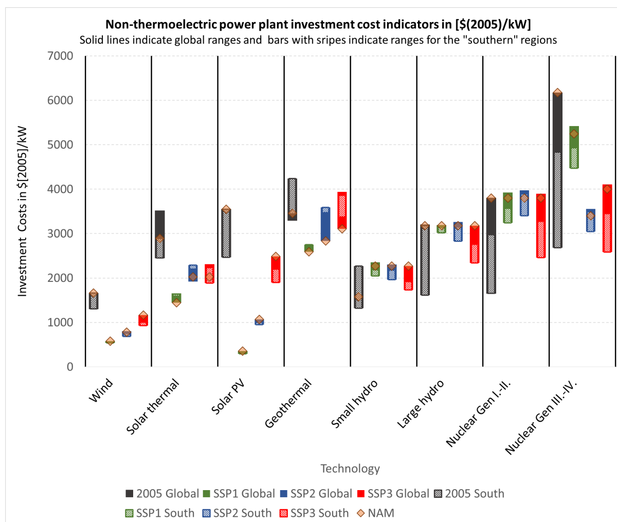
Fig. 3.7: Cost indicators for non-thermoelectric power-plant investment (Fricko et al., 2017 [[17]]). Abbreviations: CCS – Carbon Capture and Storage; IGCC – Integrated gasification combined cycles; ST – Steam turbine; CT – Combustion turbine; CCGT – Combined cycle gas turbine
